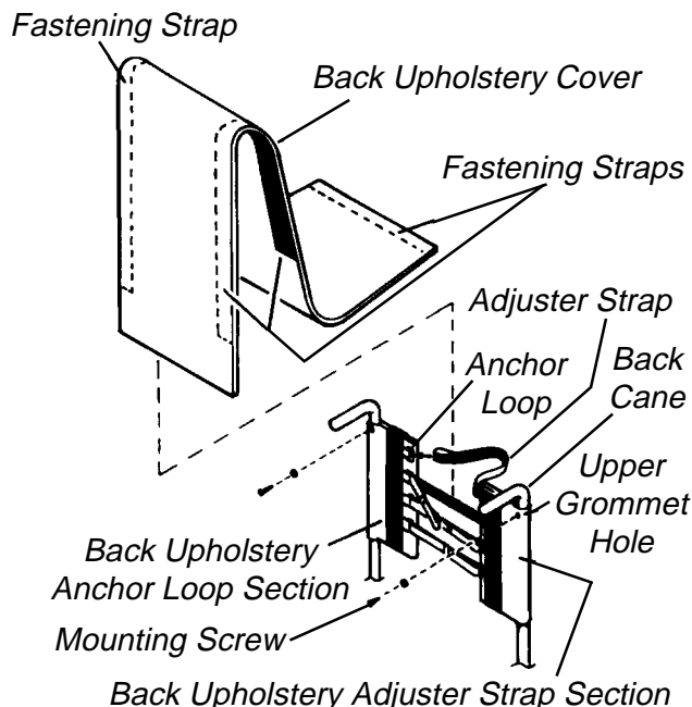
FIGURE 5 - REPLACING CUSTOM MANUAL ADJUSTABLE TENSION BACK UPHOLSTERY
